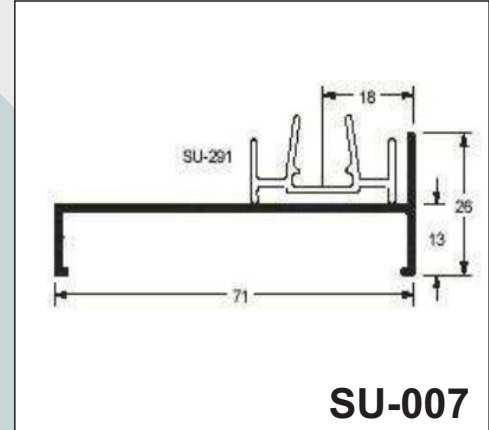
Marco Lateral
