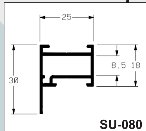
Travessa sup.
