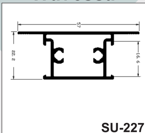
Travessa
