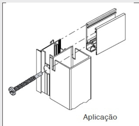
Parafuso 4,2x32
